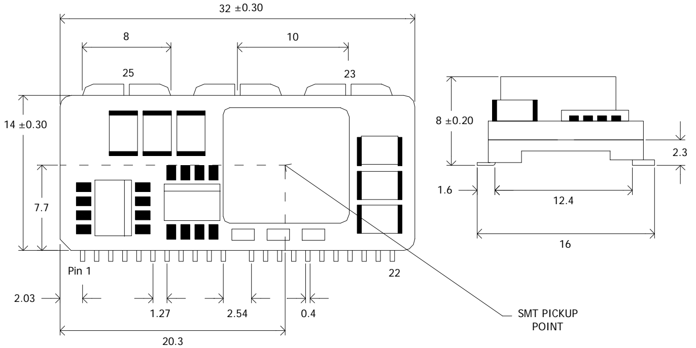
Figure 58. Mechanical Drawing
