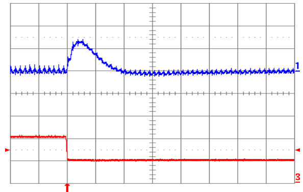
Fig. 2.0V.8: Output voltage response (YNL12S10020) to negative load current step change from 10 A to 5 A with slew rate of -5 A/ \mu\text{s} at V_{in} = 12\text{ V} . Top trace: output voltage (100 mV/div.); Bottom trace: load current (5 A/div.). C_o = 100\text{ }\mu\text{F} ceramic. Time scale: 20 \mu\text{s} /div.
