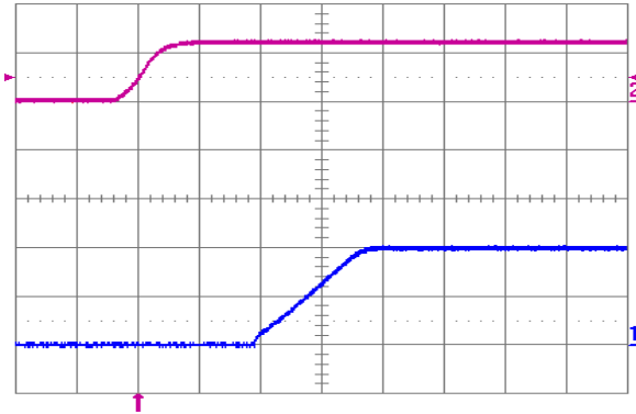
Fig. 2.0V.5: Turn-on transient (YNL12S10020) with application of V_{in} at full rated load current (resistive) and 100 \mu\text{F} external capacitance at V_{in} = 12\text{ V} . Top trace: V_{in} (10 V/div.); Bottom trace: output voltage (1 V/div.); Time scale: 2 ms/div.
