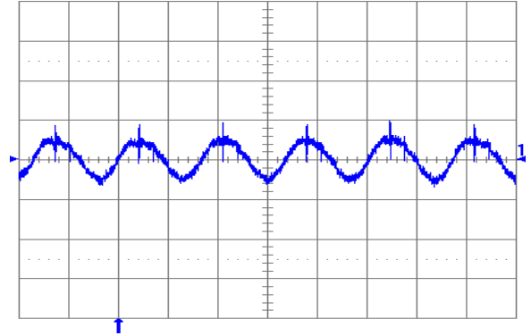
Fig. 2.0V.6: Output voltage ripple (20 mV/div.) at full rated load current into a resistive load with external capacitance 100 \mu\text{F} ceramic + 1 \mu\text{F} ceramic and V_{in} = 12\text{ V} (YNL12S10020). Time scale: 2 \mu\text{s} /div.
