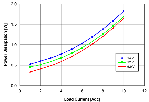
Fig. 1.5V.4: Power loss vs. load current and input voltage for YNL12S10015 converter mounted vertically with air flowing at a rate of 200 LFM (1 m/s) and T_a = 25\text{ }^{\circ}\text{C} .
