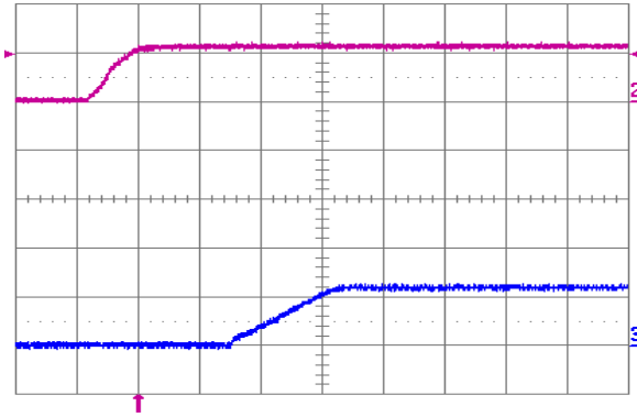
Fig. 1.2V.5: Turn-on transient (YNL12S10012) with application of V_{in} at full rated load current (resistive) and 100\ \mu\text{F} external capacitance at V_{in} = 12\ \text{V} . Top trace: V_{in} (10 V/div.); Bottom trace: output voltage (1 V/div.); Time scale: 2 ms/div.
