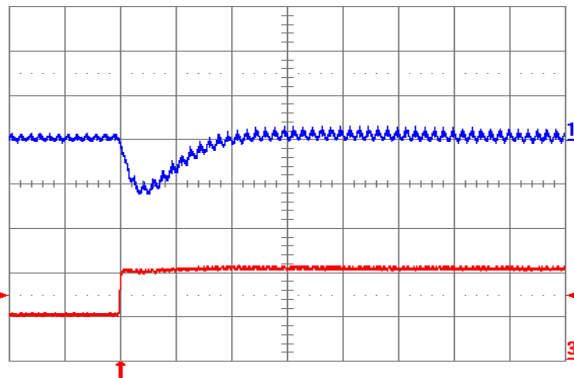
Fig. 2.0V.7: Output voltage response (YNL12S10020) to positive load current step change from 5 A to 10 A with slew rate of 5 A/ \mu\text{s} at V_{in} = 12\text{ V} . Top trace: output voltage (100 mV/div.); Bottom trace: load current (5 A/div.). C_o = 100\text{ }\mu\text{F} ceramic. Time scale: 20 \mu\text{s} /div.
