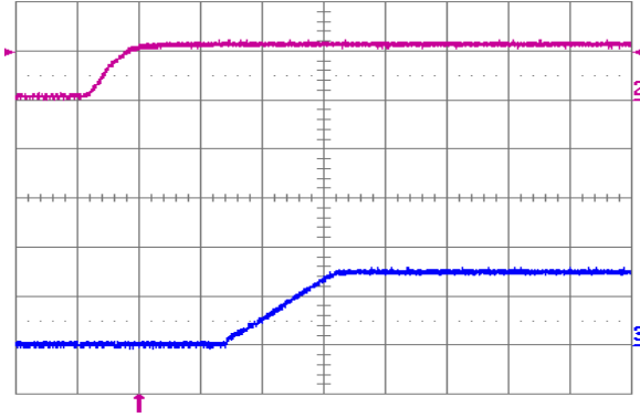
Fig. 1.5V.5: Turn-on transient (YNL12S10015) with application of V_{in} at full rated load current (resistive) and 100\ \mu\text{F} external capacitance at V_{in} = 12\ \text{V} . Top trace: V_{in} (10 V/div.); Bottom trace: output voltage (1 V/div.); Time scale: 2 ms/div.
