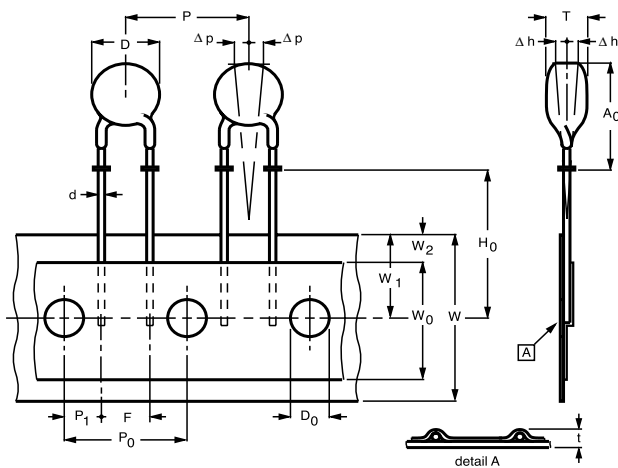
For dimensions, see Taping data table
