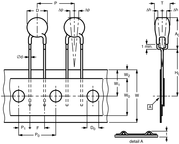
For dimensions, see Taping data table
