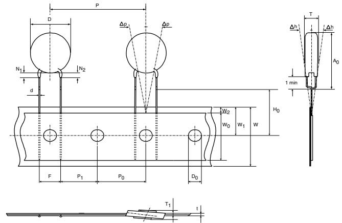
For dimensions, see Taping data table
