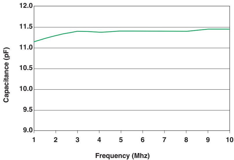
Figure 2. I/O Capacitance vs Frequency (Typical Values)
