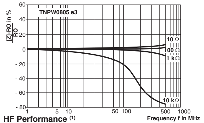
HF Performance (1)
