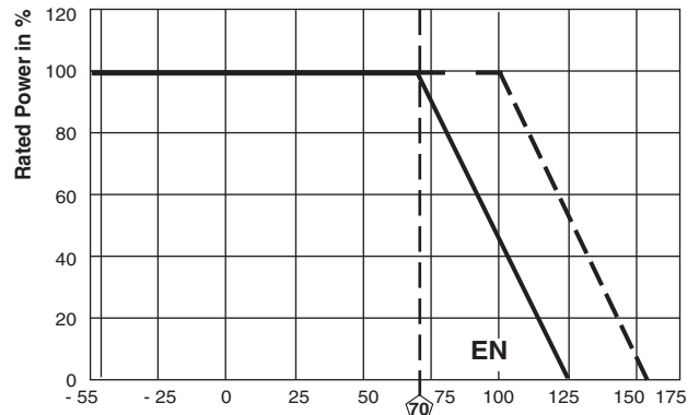
Derating
