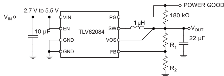
Figure 10. Typical Application Circuit
