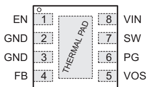
8-Terminal SON With Thermal Pad DSG Package (Top View)
