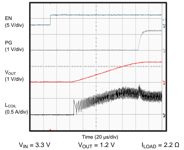
Figure 16. Startup
