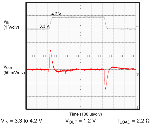
Figure 15. Line Transient
