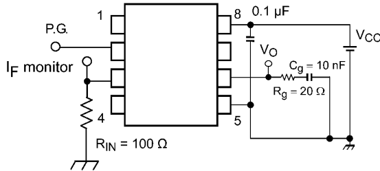
Fig. 12.1.7 Switching Time Test Circuit
