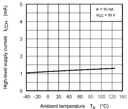
Fig. 12.2.6 I CCH - T a
