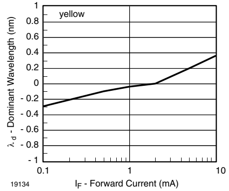
Fig. 9 - Dominant Wavelength vs. Forward Current
