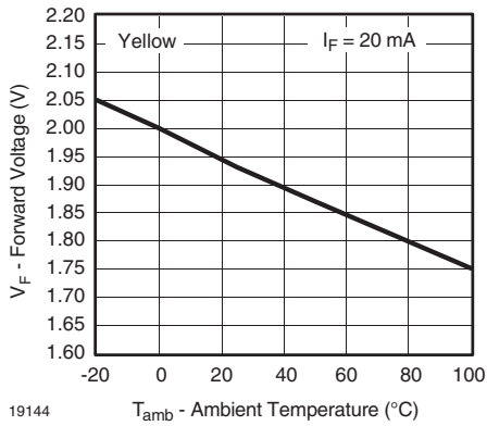
Figure 13. Forward Voltage vs. Ambient Temperature
