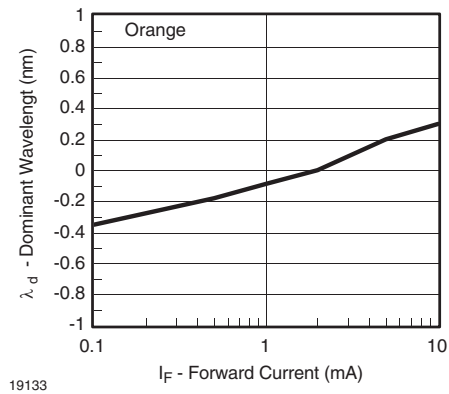
Figure 4. Dominant Wavelength vs. Forward Current
