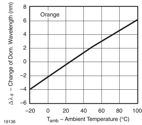
Figure 5. Change of Dominant Wavelength vs. Ambient Temperature
