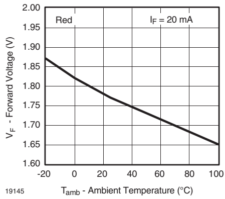
Figure 19. Forward Voltage vs. Ambient Temperature
