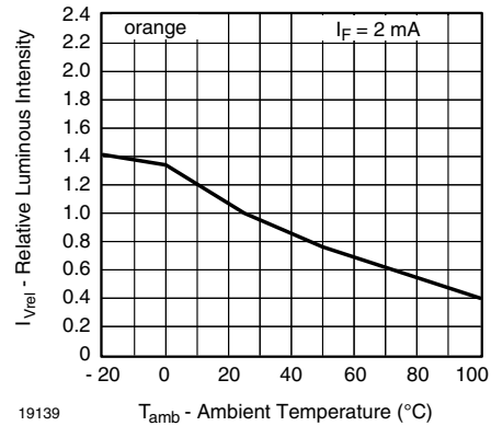
Figure 5. Relative Luminous Intensity vs. Ambient Temperature
