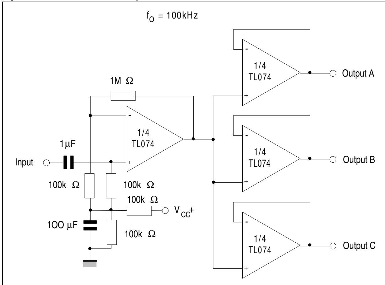
Figure 20. Audio distribution amplifier
