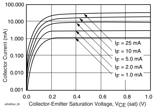
Figure 6. Collector Current vs. Collector-Emitter Saturation Voltage
