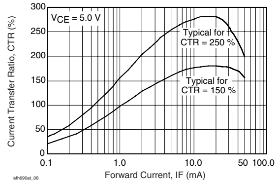
Figure 9. Current Transfer Ratio vs. Forward Current
