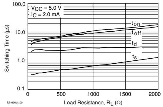
Figure 10. Switching Time vs. Load Resistance
