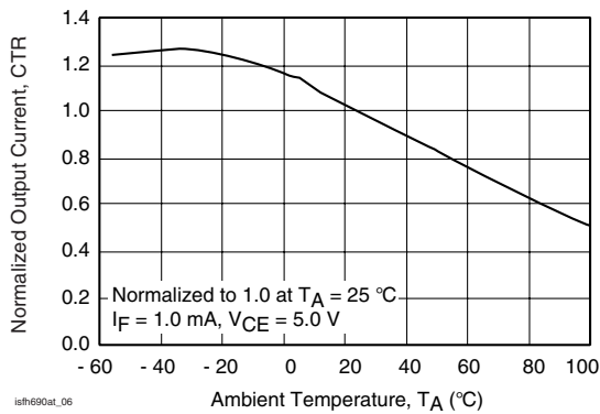
Figure 7. Normalized Output Current vs. Ambient Temperature
