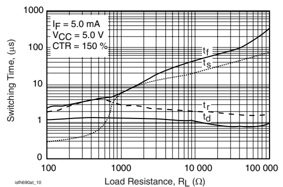
Figure 11. Switching Time vs. Load Resistance
