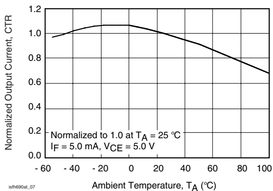
Figure 8. Normalized Output Current vs. Ambient Temperature
