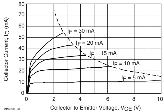
Figure 4. Collector Current vs. Collector Emitter Voltage
