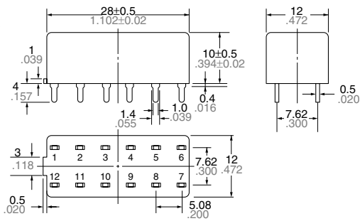
External dimensions
