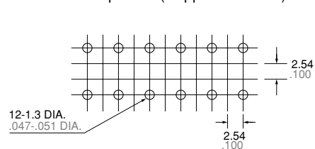
PC board pattern (Copper-side view)
