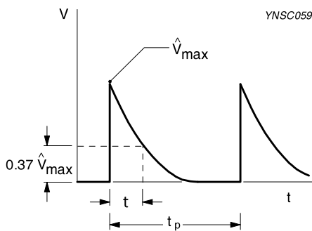
Fig. 15 Exponential pulses
