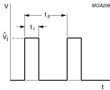
Fig. 14 Rectangular pulses
