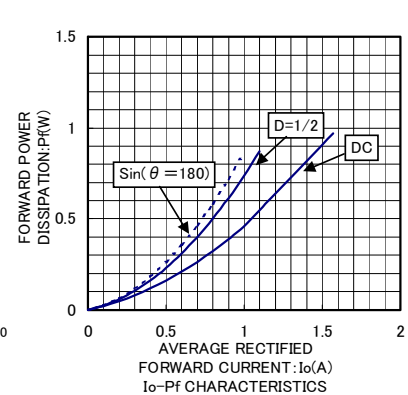
Io-Pf CHARACTERISTICS
