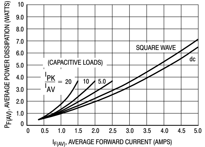
Figure 8. Power Dissipation
