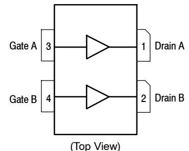
CASE 2282-02 NI-1230S-4 GULL MRFE6VP61K25GSR5
