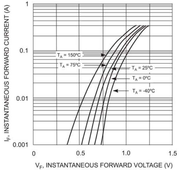
Fig. 2 Forward Characteristics
