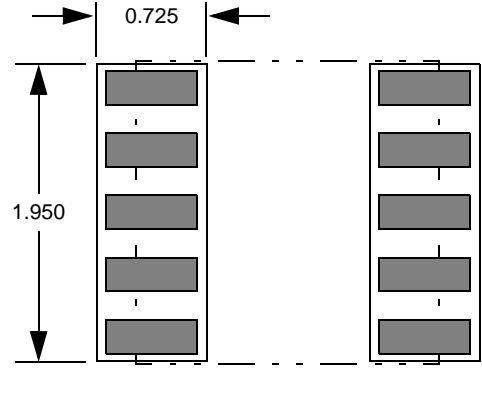
Figure 7. Footprints and Soldering Masks (dimensions in mm)
