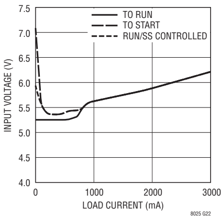
Minimum Input Voltage vs Load Current, 5V_{OUT}
