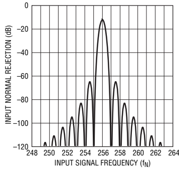
Figure 29. Input Normal Mode Rejection 2x Speed Mode
