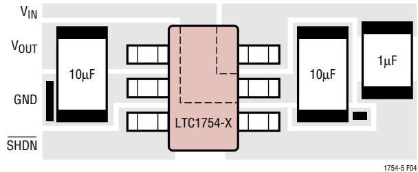
Figure 4. Recommended Layout
