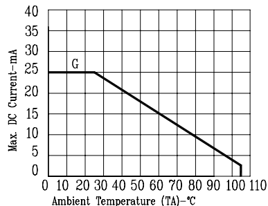
Fig5. MAX. ALLOWABLE DC CURRENT VS. AMBIENT TEMPERATURE.
