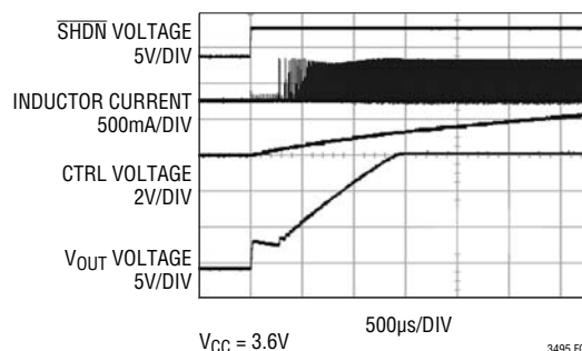
Figure 5. Soft-Start Waveform
