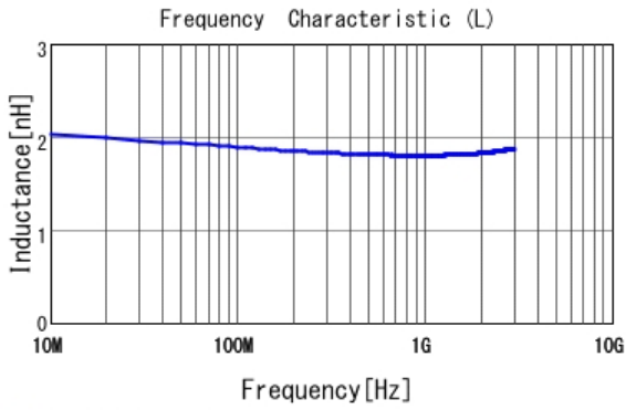
■ LQP03TN1N8C02 L
