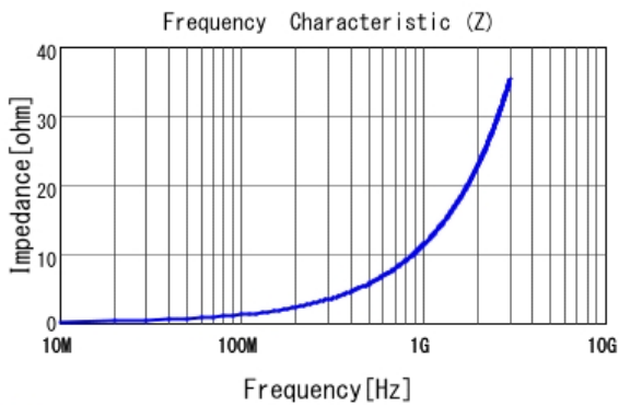
■ LQP03TN1N8C02 |Z|
