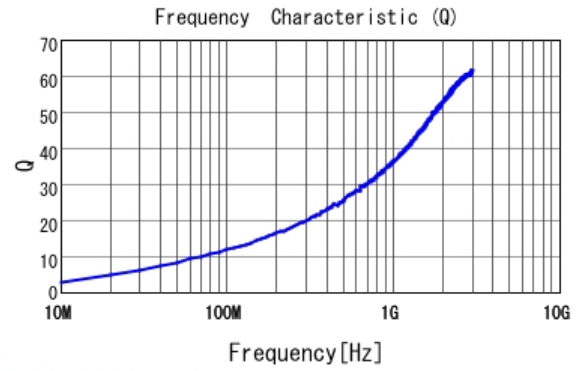
■ LQP03TN1N8C02 Q
