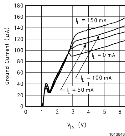
Ground Current vs V_IN @ 25°C
