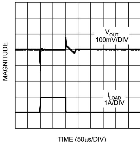
Load Transient Response (Tantalum 10 \mu\text{F}/1\text{A} )
