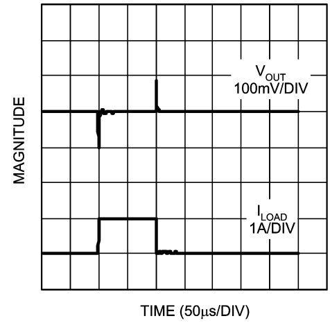
Load Transient Response (SANYO 150 \mu\text{F}/1\text{A} )
