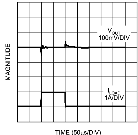
Load Transient Response (Tantalum 100 \mu\text{F}/1\text{A} )
