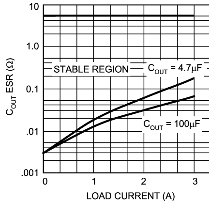
20062431 Minimum ESR vs Output Load Current
