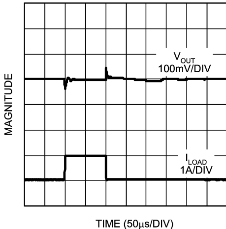
Load Transient Response (Both POSCAP 100 \mu\text{F}/1\text{A} )
