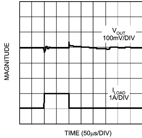
Load Transient Response (Both Oscon 100 \mu\text{F}/1\text{A} )
