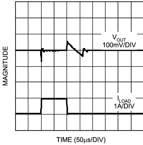
Load Transient Response (Both Oscon 10 \mu\text{F}/1\text{A} )
