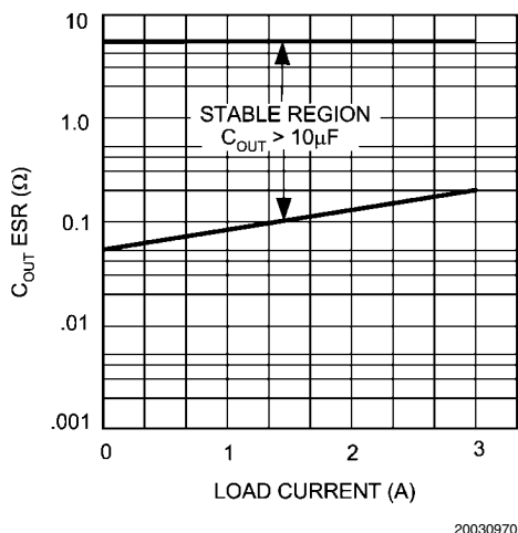
FIGURE 1. ESR Curve for C_{OUT} (with 10\mu\text{F} Tantalum Input Capacitor)
