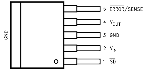
Top View TO263-5 Package
