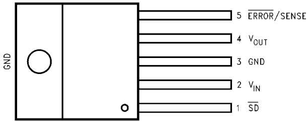
Top View TO220-5 Package Bent, Staggered Leads
