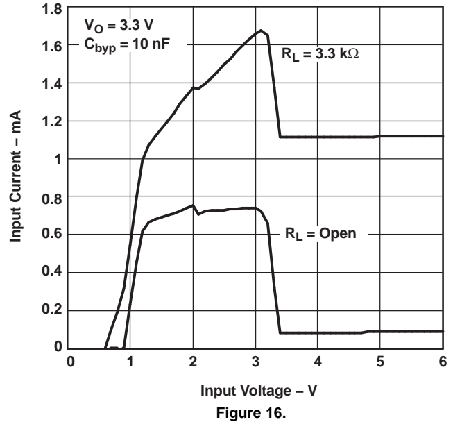
INPUT CURRENT vs INPUT VOLTAGE
