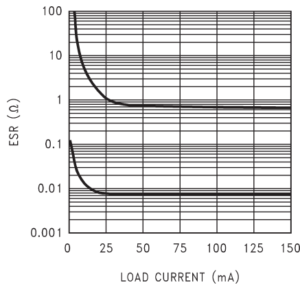
Figure 28. 2.2-μF Stable ESR Range for Output Voltage ≤2.3 V
