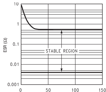
Figure 30. 2.2-μF/3.3-μF Stable ESR Range for Output Voltage ≥2.5 V
