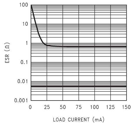
Figure 29. 4.7-μF Stable ESR Range for Output Voltage ≤2.3 V
