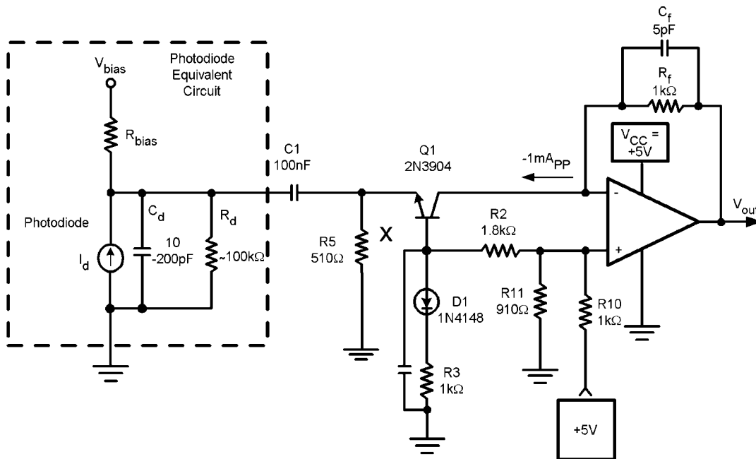
FIGURE 4. Single Supply Photodiode I-V Converter
