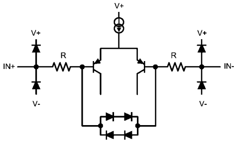
FIGURE 3. Input Equivalent Circuit
