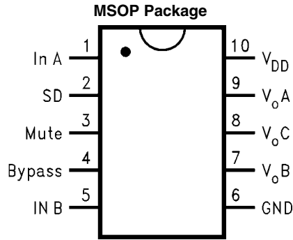
20031479 Top View Order Number LM4911/LM4911QMM See NS Package Number MUB10A
