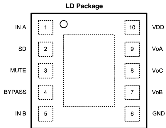
200314c0 Top View Order Number LM4911 See NS Package Number LDA10A
