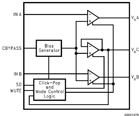
FIGURE 1. Block Diagram
