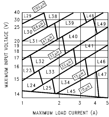
FIGURE 5. LM2677-12
