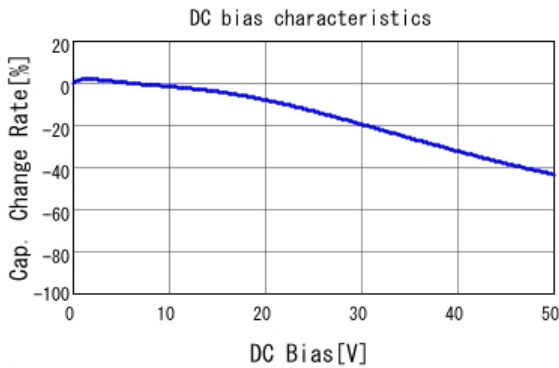
■ GRM32RR71H105KA01 C-DC bias capchange, 25.0degC, AC1.
