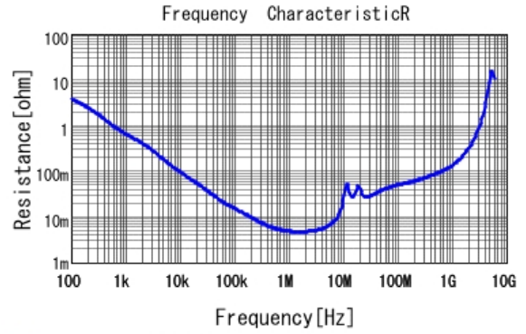
■ GRM32RR71H105KA01 R DCOV, 25degC
