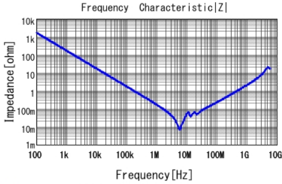
■ GRM32RR71H105KA01 |Z| DCOV, 25degC
