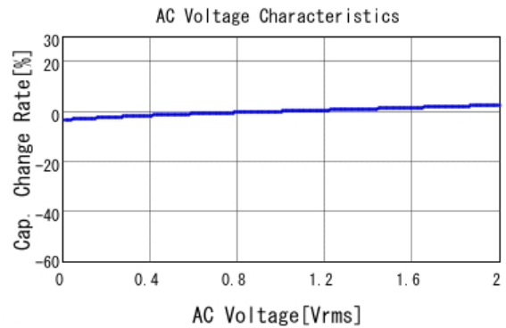
■ GRM32RR71H105KA01 C-AC Voltage capchange, DCOV, 25.0d
