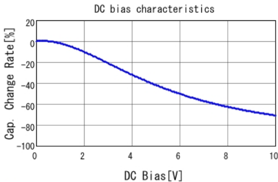
■ GRM32ED71A476ME15 C-DC bias capchange, 25.0degC, AC0.
