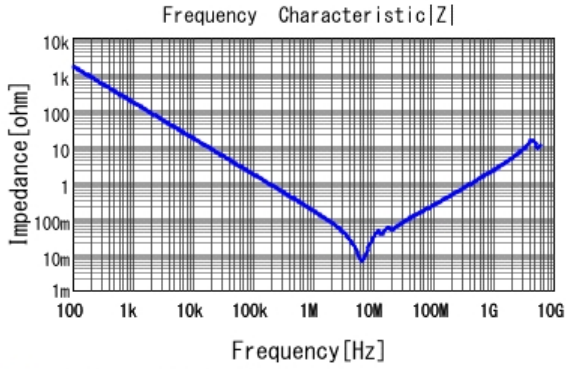
■ GRM21BR71H105KA12 |Z| DCOV, 25degC
