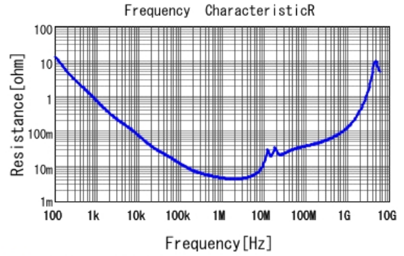
■ GRM21BR71H105KA12 R DCOV, 25degC
