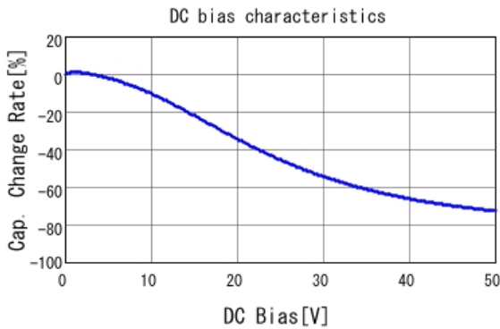
■ GRM21BR71H105KA12 C-DC bias capchange, 25.0degC, AC1.
