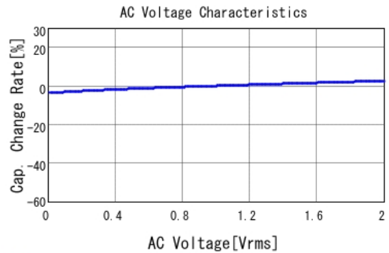
■ GRM21BR71H105KA12 C-AC Voltage capchange, DCOV, 25.0d
