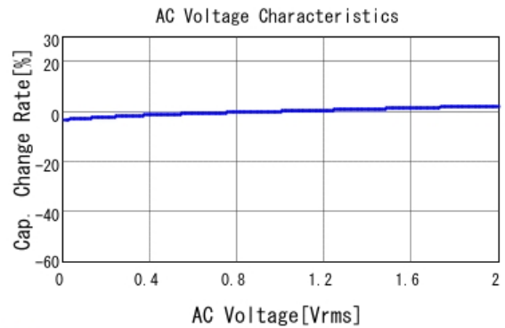
■ GRM21BR71E104KA01 C-AC Voltage capchange, DCOV, 25.0d
