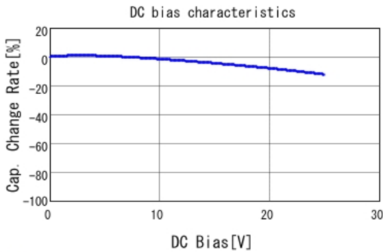
■ GRM21BR71E104KA01 C-DC bias capchange, 25.0degC, AC1.
