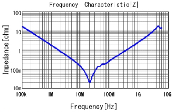
■ GRM21BR71E104KA01 |Z| DCOV, 25degC
