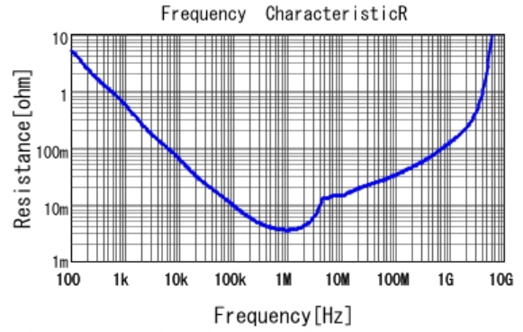
■ GRM21BR61E106KA73 R DCOV, 25degC
