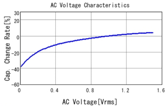
■ GRM21BR61E106KA73 C-AC Voltage capchange, DCOV, 25.0d
