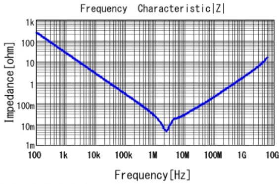
■ GRM21BR61E106KA73 |Z| DCOV, 25degC
