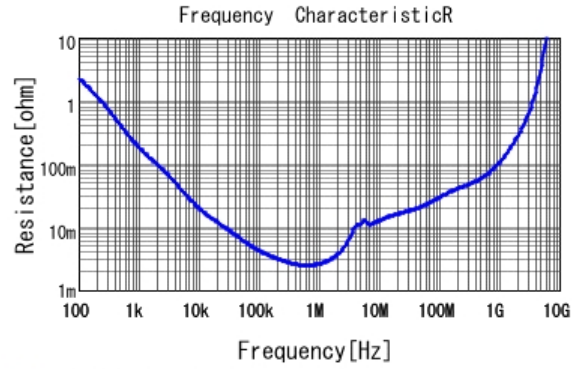
■ GRM21BR61C106KE15 R DCOV, 25degC
