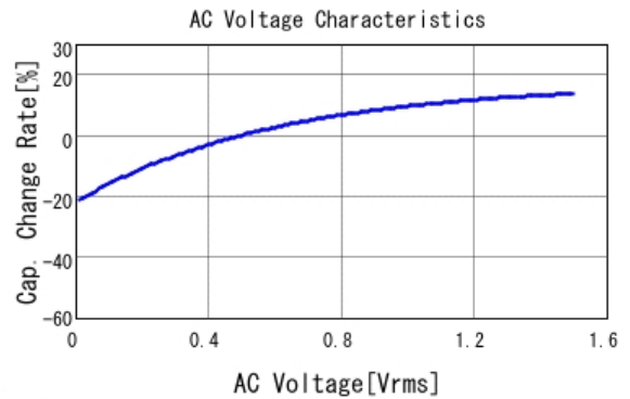
■ GRM21BR61C106KE15 C-AC Voltage capchange, DCOV, 25.0d
