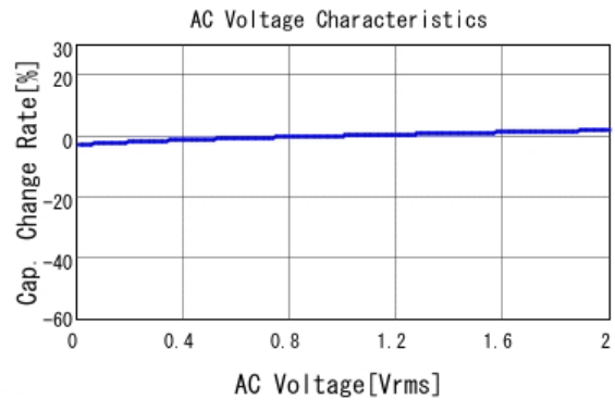
■ GRM216R71H103KA01 C-AC Voltage capchange, DCOV, 25.0d
