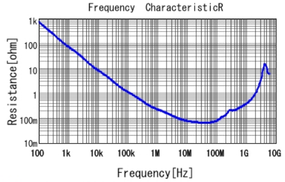
■ GRM216R71H103KA01 R DCOV, 25degC
