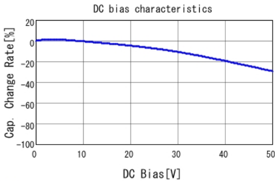
■ GRM216R71H103KA01 C-DC bias capchange, 25.0degC, AC1.
