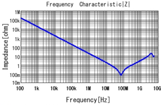
■ GRM216R71H103KA01 |Z| DCOV, 25degC
