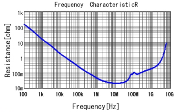
■ GRM188R71H473KA61 R DCOV, 25degC
