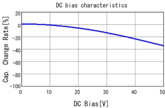
■ GRM188R71H473KA61 C-DC bias capchange, 25.0degC, AC1.
