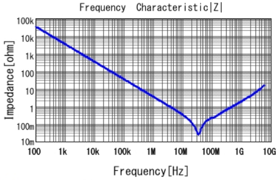
■ GRM188R71H473KA61 |Z| DCOV, 25degC
