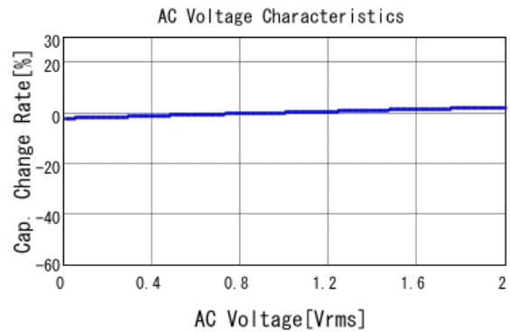
■ GRM188R71H473KA61 C-AC Voltage capchange, DCOV, 25.0d
