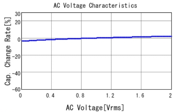
■ GRM188R71H103KA01 C-AC Voltage capchange, DCOV, 25.0d
