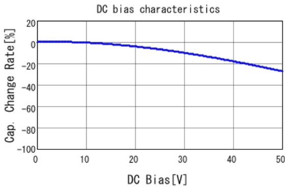
■ GRM188R71H103KA01 C-DC bias capchange, 25.0degC, AC1.
