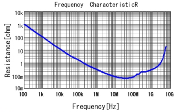
■ GRM188R71H103KA01 R DCOV, 25degC
