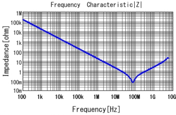
■ GRM188R71H103KA01 |Z| DCOV, 25degC
