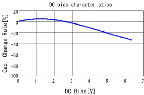
■ GRM188R70J105KA01 C-DC bias capchange, 25.0degC, AC1.
