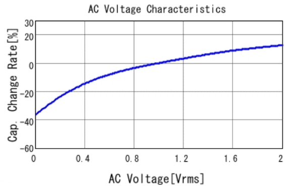
■ GRM188R70J105KA01 C-AC Voltage capchange, DCOV, 25.0d
