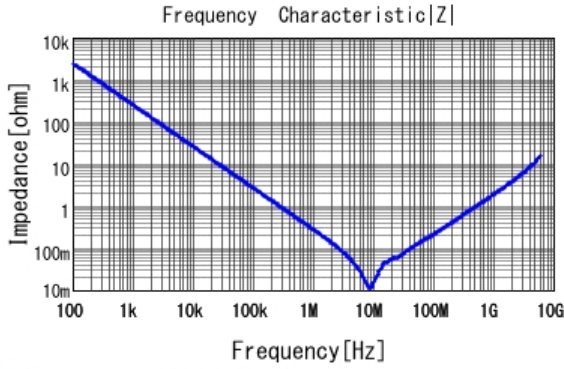
■ GRM188R70J105KA01 |Z| DCOV, 25degC
