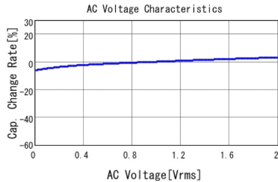
■ GRM188R70J104KA01 C-AC Voltage capchange, DCOV, 25.0d
