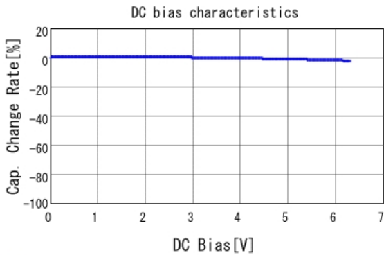
■ GRM188R70J104KA01 C-DC bias capchange, 25.0degC, AC1.
