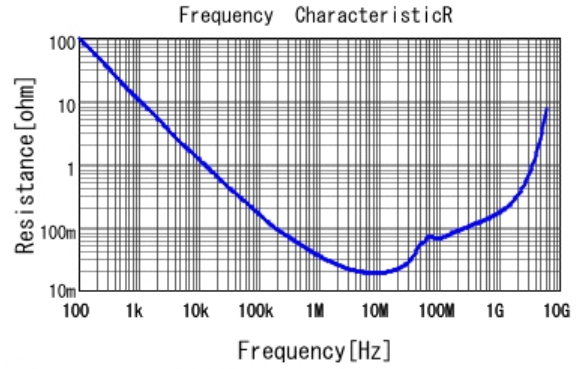
■ GRM188R70J104KA01 R DCOV, 25degC
