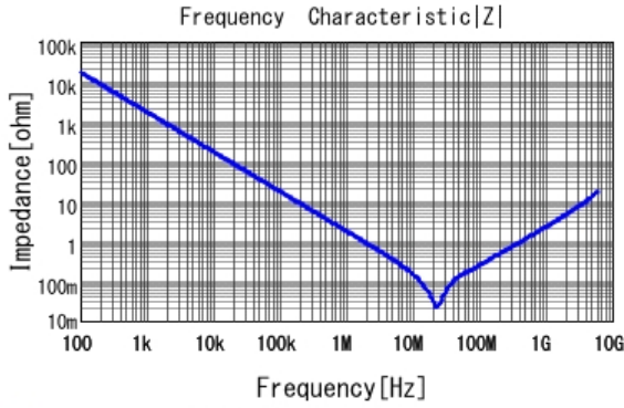
■ GRM188R70J104KA01 |Z| DCOV, 25degC
