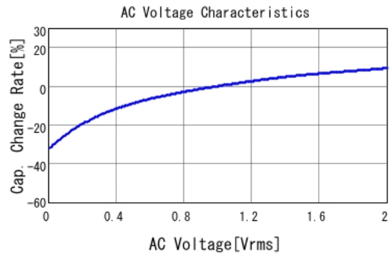
■ GRM188R61E105KA12 C-AC Voltage capchange, DCOV, 25.0d
