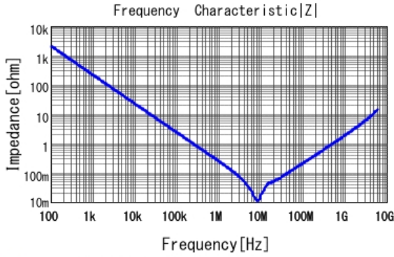
■ GRM188R61E105KA12 |Z| DCOV, 25degC
