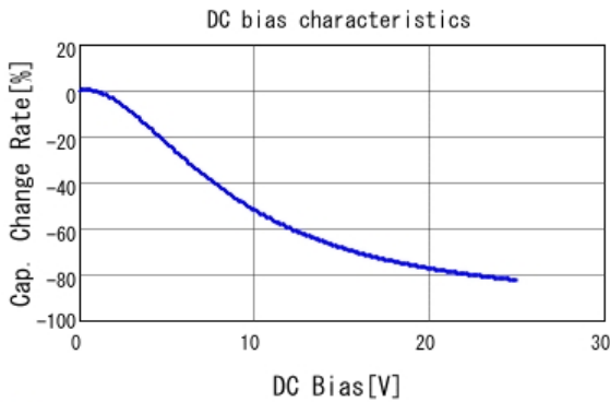
■ GRM188R61E105KA12 C-DC bias capchange, 25.0degC, AC1.
