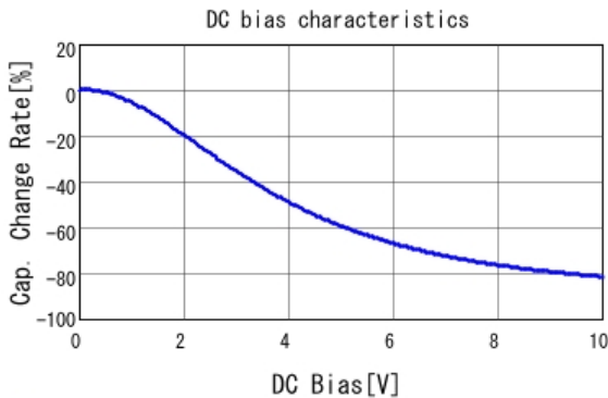
■ GRM188D71A106MA73 C-DC bias capchange, 25.0degC, AC1V
