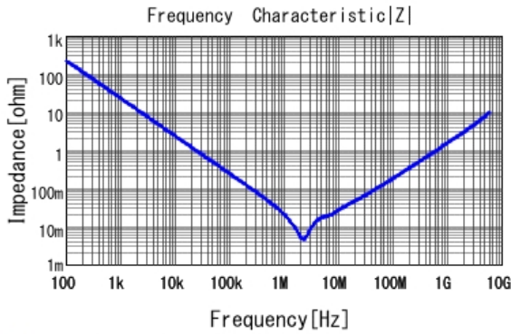
■ GRM188D71A106MA73 |Z| DCOV, 25degC
