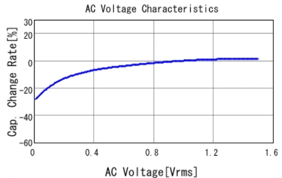
■ GRM188D71A106MA73 C-AC Voltage capchange, DCOV, 25.0d
