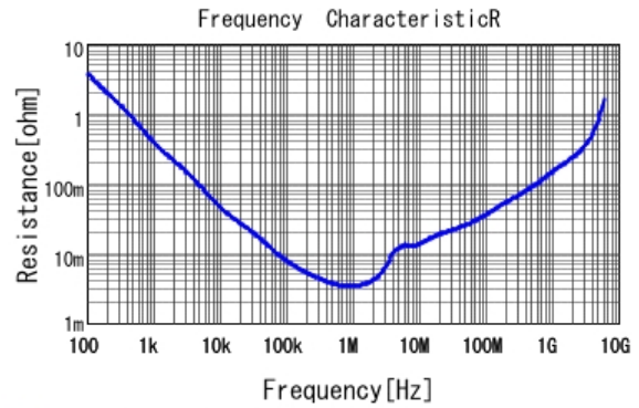
■ GRM188D71A106MA73 R DCOV, 25degC
